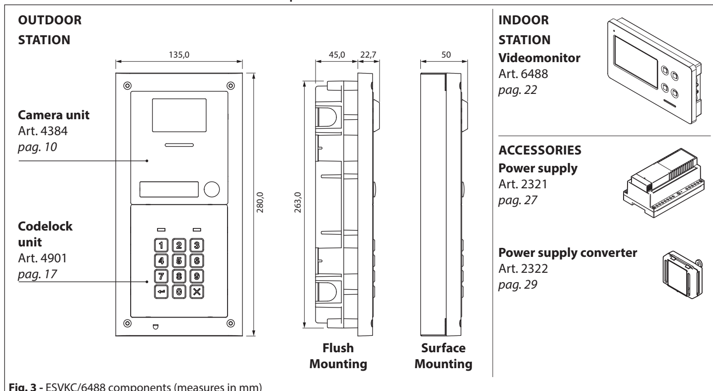
Fig. 3 - ESVKC/6488 components (measures in mm)
