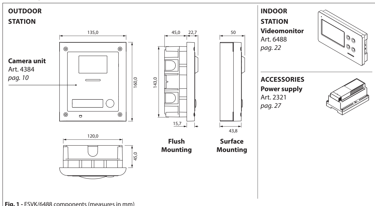
Fig. 1 - ESVK/6488 components (measures in mm)
